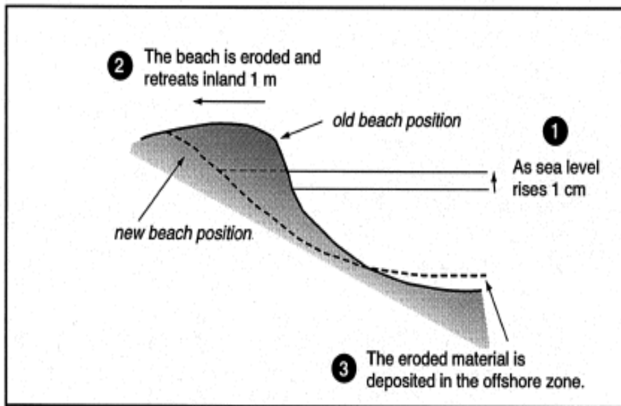
Figure 2 Beach Retreat due to Sea Level Rise (Cambers, 1997)
